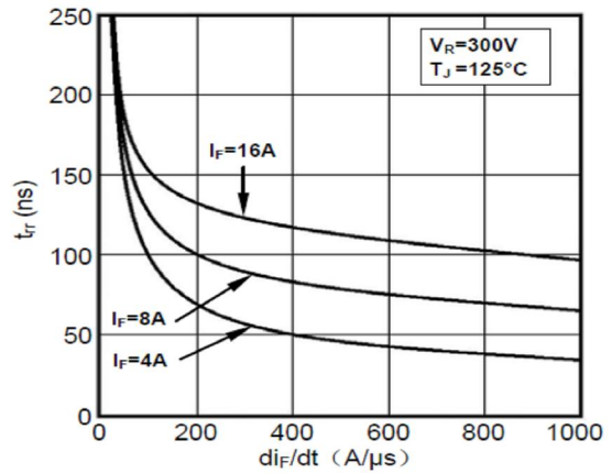
Fig2. Reverse Recovery Time vs di_F/dt
