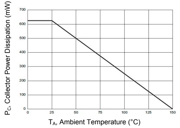
Figure 8. Power Derating
