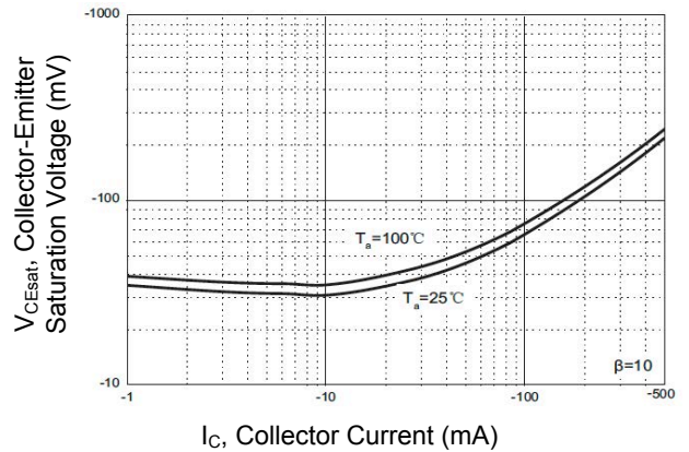
Figure 4. Collector Emitter Saturation Voltage vs. Ic
