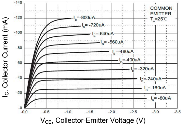
Figure 1. Static Characteristic
